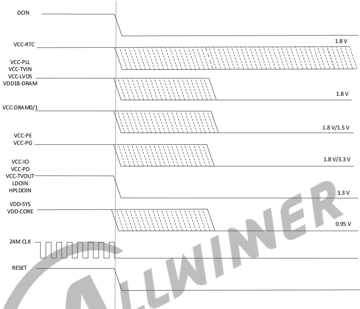
Figure 5-29 Power-Off Timing
