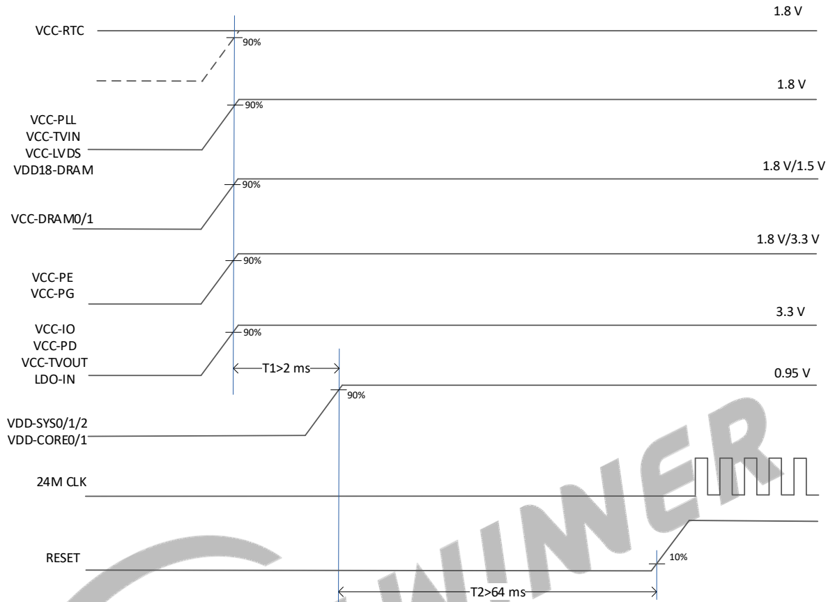
Figure 5-28 Power-On Timing
