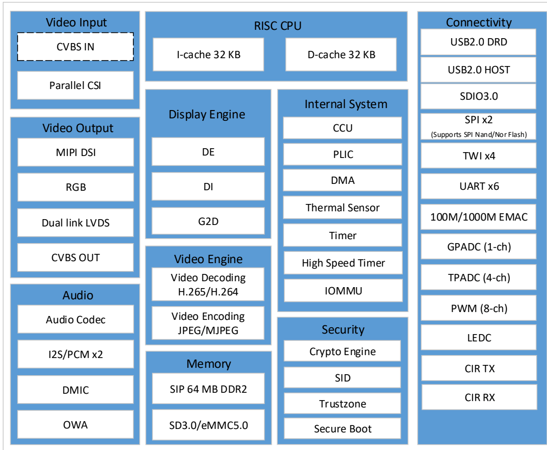
Figure 3-1 F133 System Block Diagram
