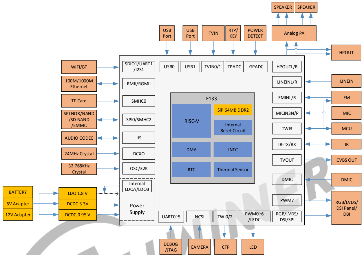
Figure 3-2 F133 Decoding Platform Solution
