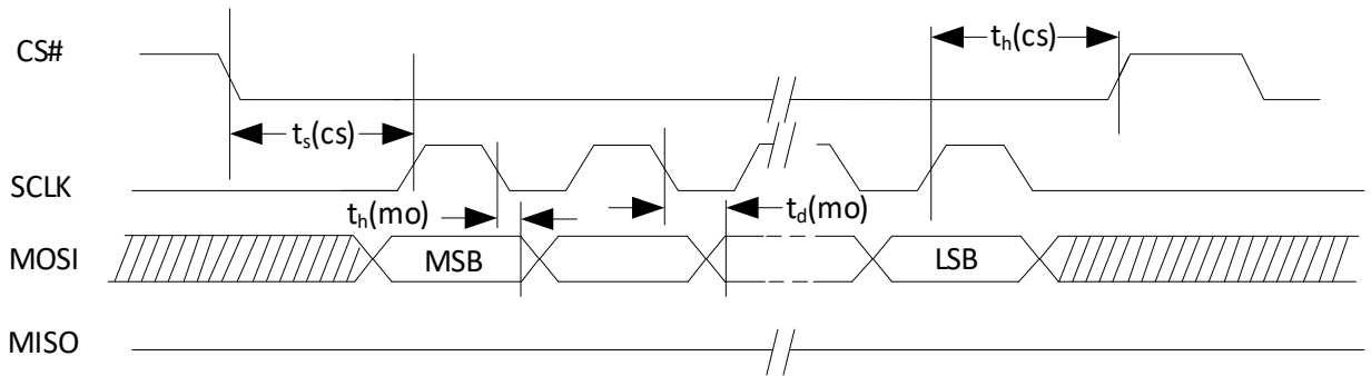
Figure 5-16 SPI Reading Timing
